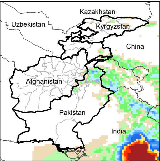
Daily Precip. Forecast for 6 Aug., 2023
