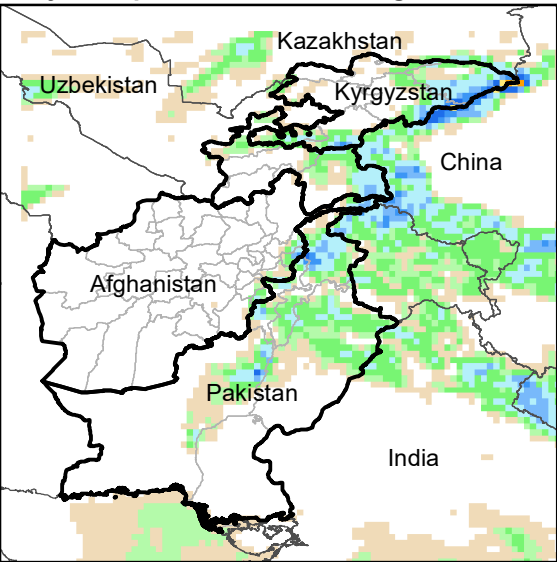
Daily Precip. Forecast for 29 Aug., 2023
