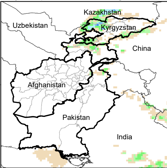
Daily Precip. Forecast for 3 Sep., 2023
