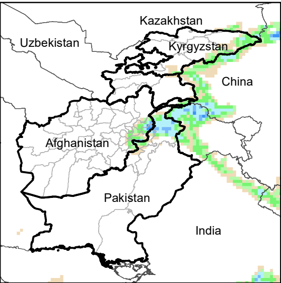
Daily Precip. Forecast for 5 Sep., 2023
