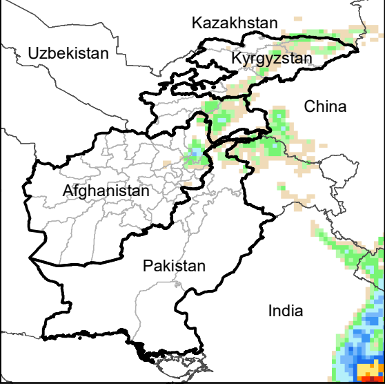
Daily Precip. Forecast for 2 Oct., 2023
