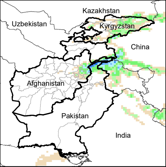
Daily Precip. Forecast for 8 Oct., 2023
