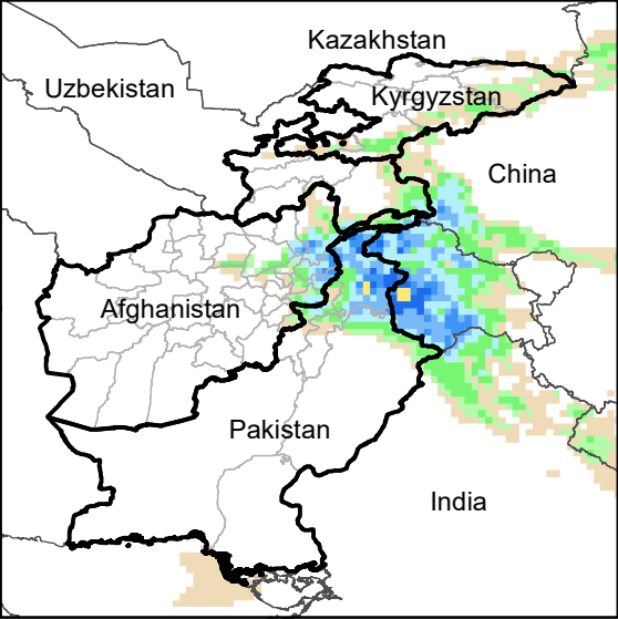
Daily Precip. Forecast for 9 Oct., 2023
