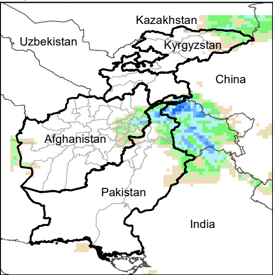
Daily Precip. Forecast for 17 Oct., 2023
