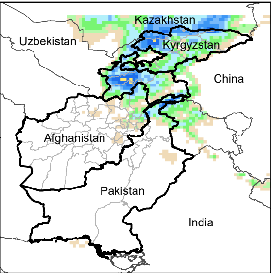
Daily Precip. Forecast for 16 Oct., 2023
