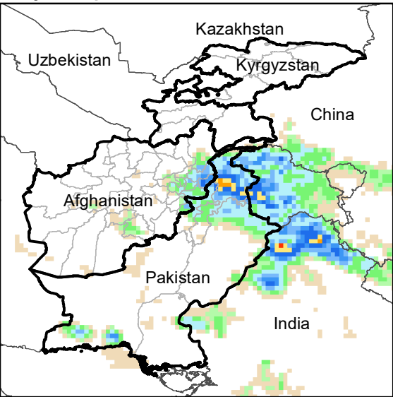
Daily Precip. Forecast for 18 Oct., 2023
