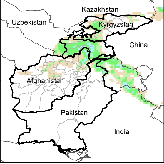
Daily Precip. Forecast for 30 Dec., 2023
