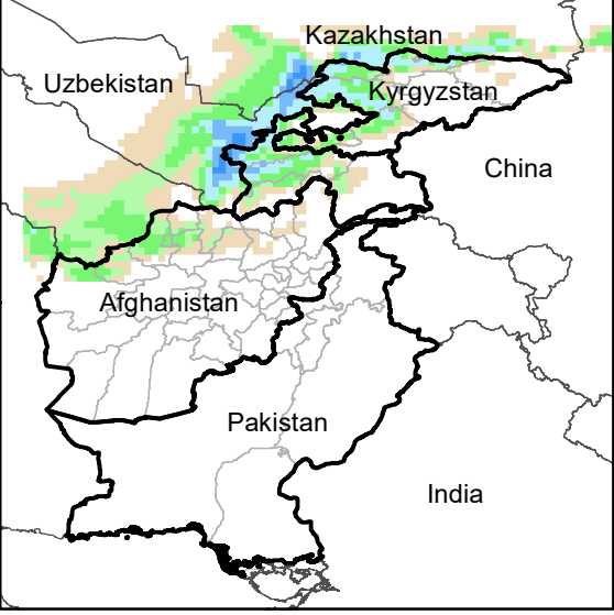
Daily Precip. Forecast for 29 Dec., 2023
