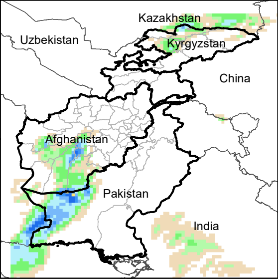
Daily Precip. Forecast for 8 Jan., 2024
