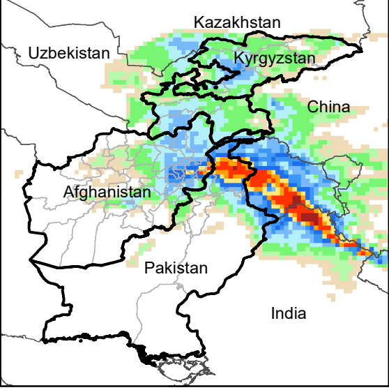
Daily Precip. Forecast for 19 Feb., 2024
