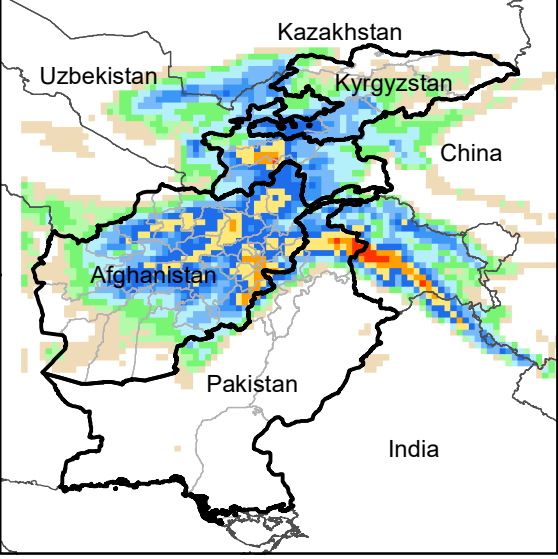
Daily Precip. Forecast for 18 Feb., 2024
