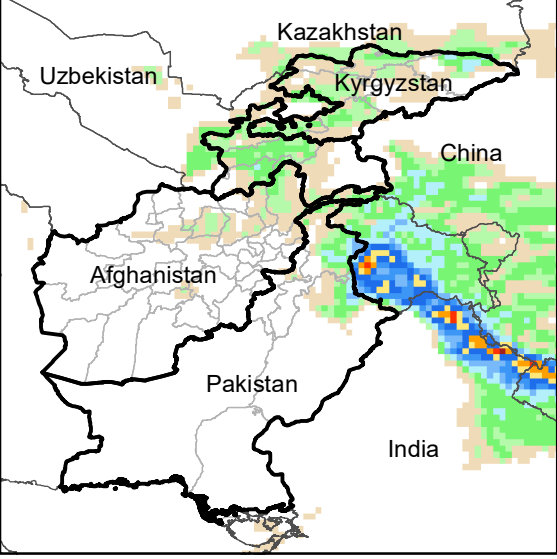
Daily Precip. Forecast for 20 Feb., 2024
