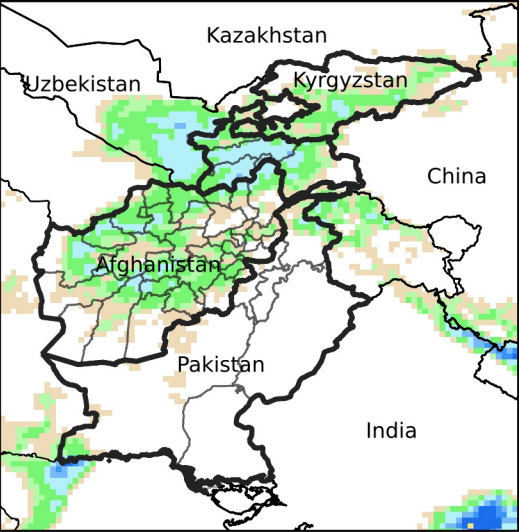
Daily Precip. Forecast for Feb 27, 2024
