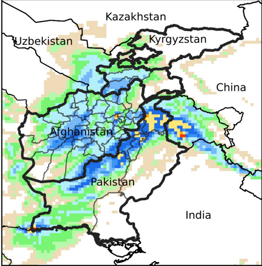
Daily Precip. Forecast for Mar 1, 2024
