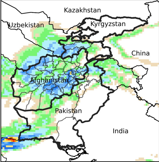
Daily Precip. Forecast for Feb 29, 2024
