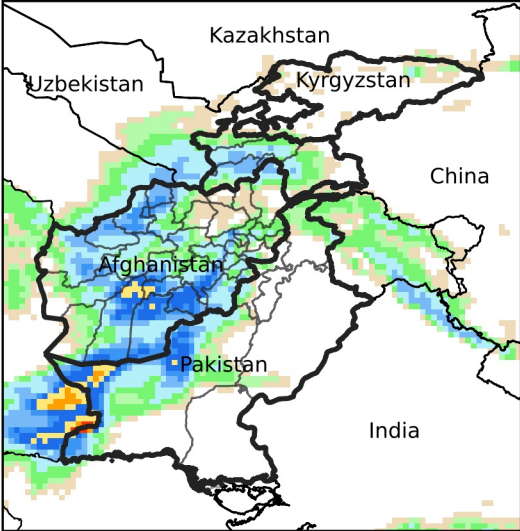
Daily Precip. Forecast for Feb 29, 2024
