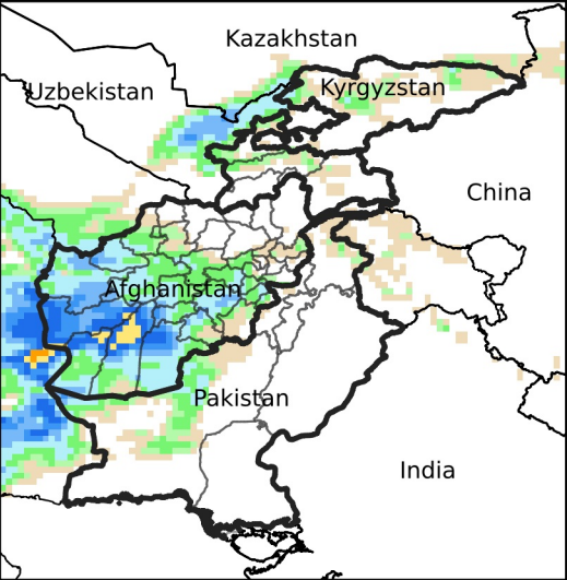
Daily Precip. Forecast for Feb 28, 2024
