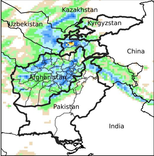
Daily Precip. Forecast for Mar 11, 2024
