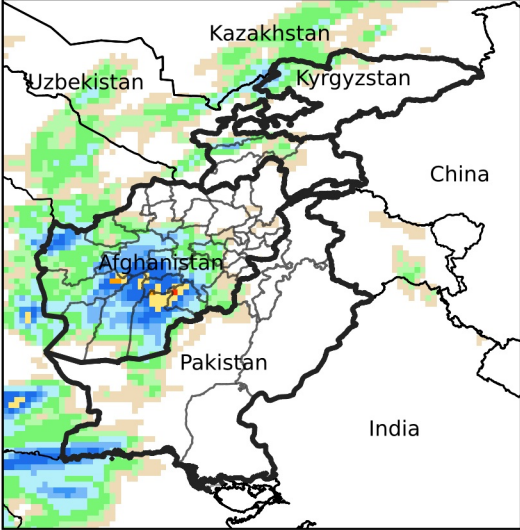
Daily Precip. Forecast for Mar 10, 2024
