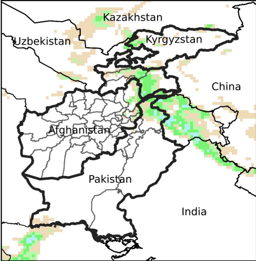
Daily Precip. Forecast for Mar 10, 2024
