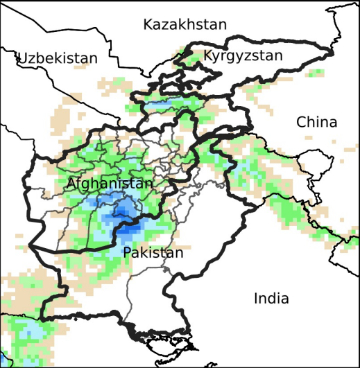
Daily Precip. Forecast for Mar 9, 2024
