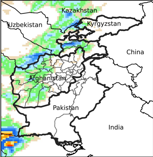
Daily Precip. Forecast for Mar 12, 2024
