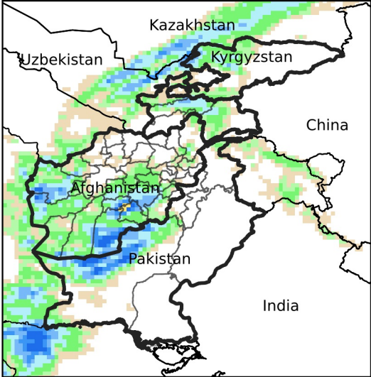
Daily Precip. Forecast for Mar 13, 2024
