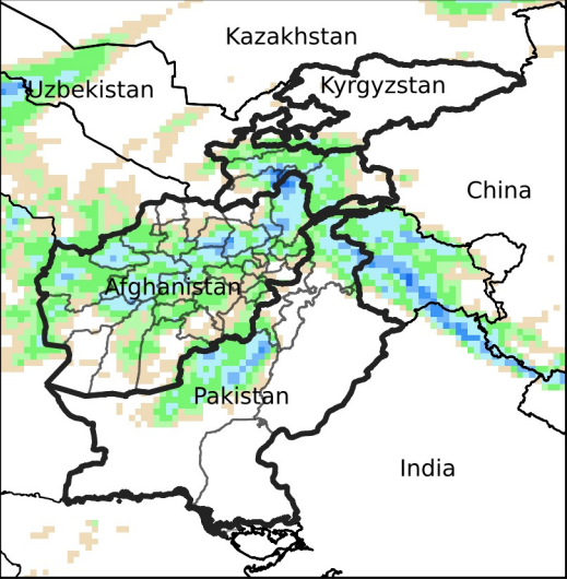
Daily Precip. Forecast for Mar 11, 2024
