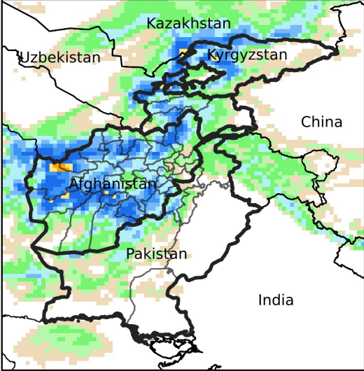
Daily Precip. Forecast for Mar 12, 2024
