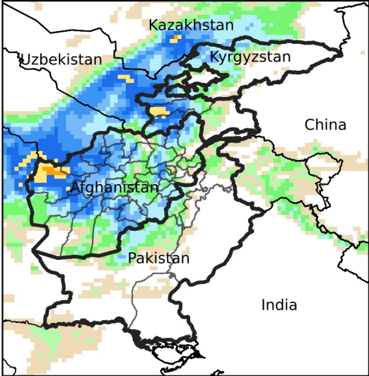
Daily Precip. Forecast for Mar 15, 2024
