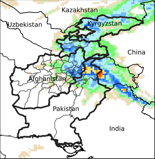
Daily Precip. Forecast for Mar 13, 2024
