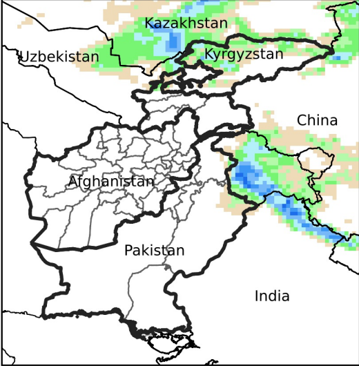
Daily Precip. Forecast for Mar 14, 2024
