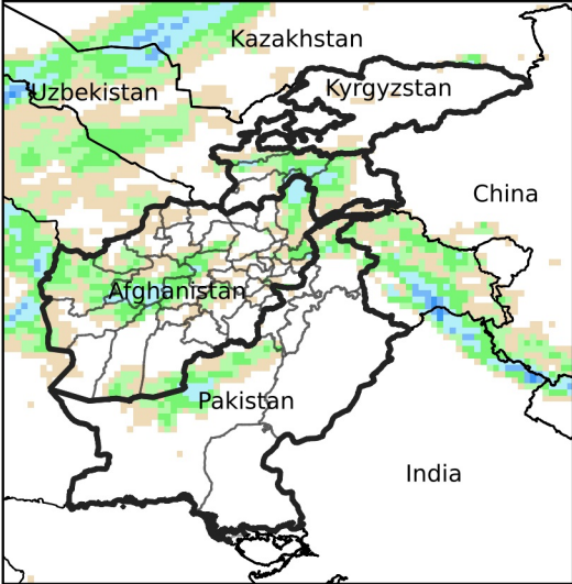
Daily Precip. Forecast for Mar 14, 2024
