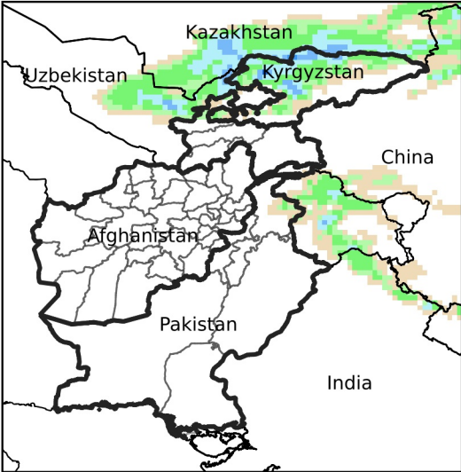
Daily Precip. Forecast for Mar 17, 2024
