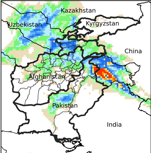
Daily Precip. Forecast for Mar 28, 2024
