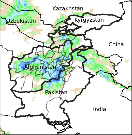
Daily Precip. Forecast for Mar 27, 2024
