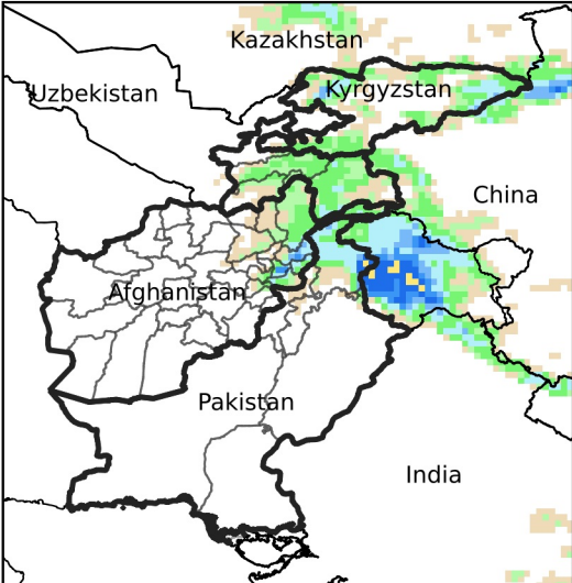
Daily Precip. Forecast for Mar 31, 2024
