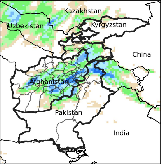
Daily Precip. Forecast for Mar 30, 2024
