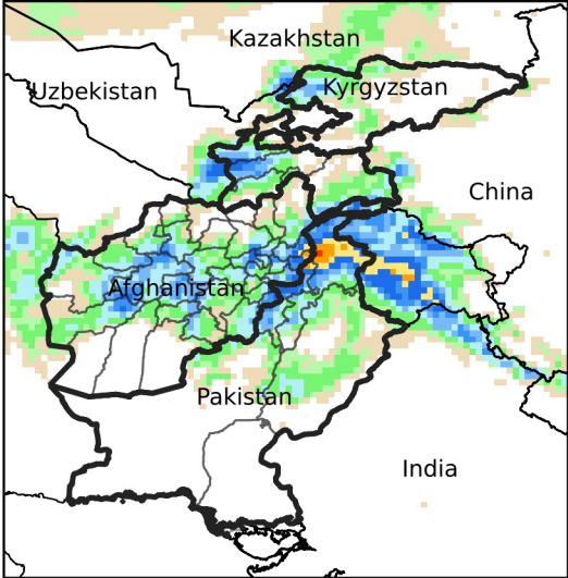
Daily Precip. Forecast for Apr 1, 2024
