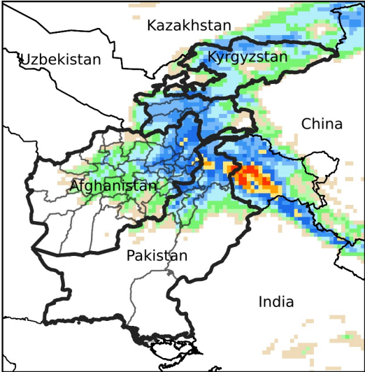
Daily Precip. Forecast for Apr 2, 2024
