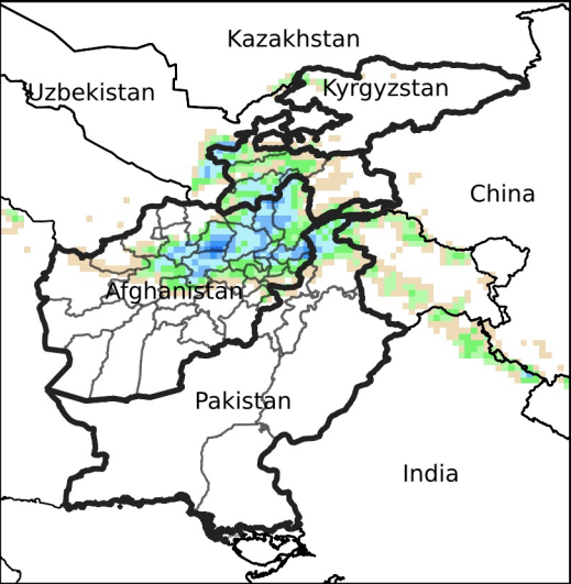
Daily Precip. Forecast for Apr 5, 2024
