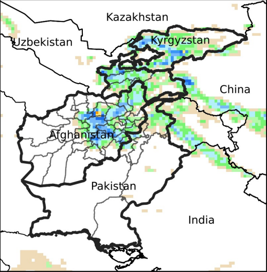
Daily Precip. Forecast for Apr 21, 2024
