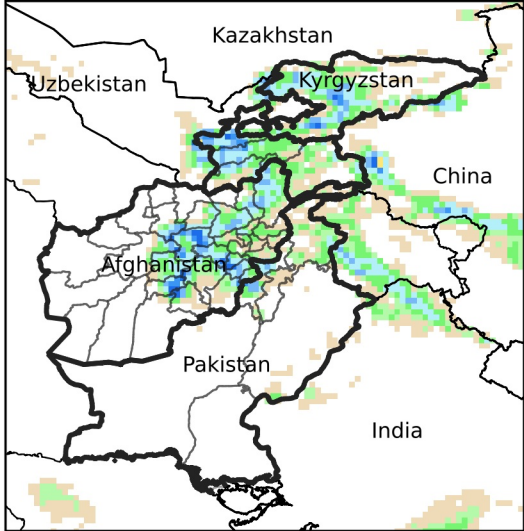
Daily Precip. Forecast for Apr 24, 2024
