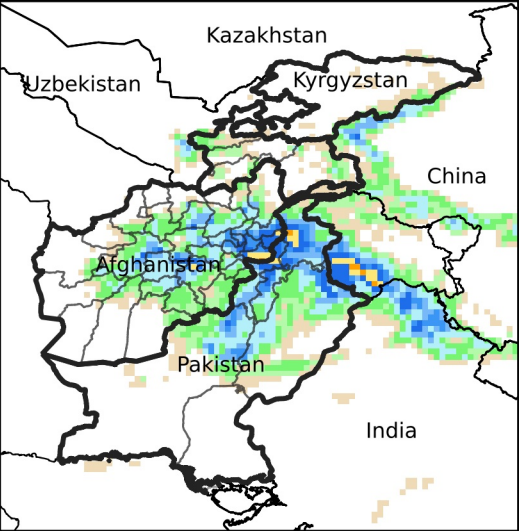
Daily Precip. Forecast for Apr 22, 2024
