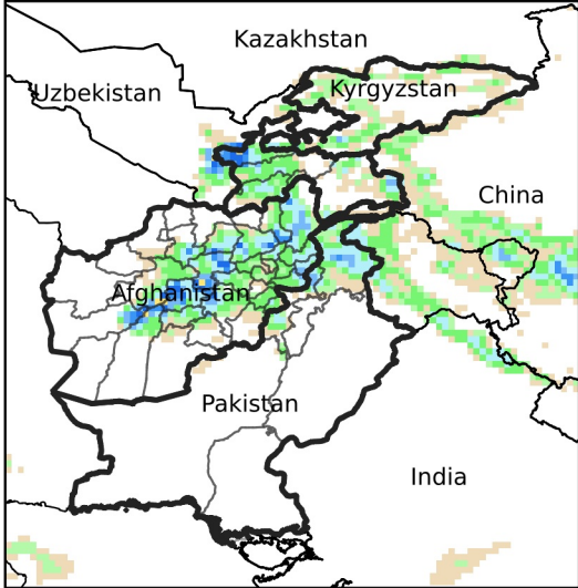
Daily Precip. Forecast for Apr 23, 2024
