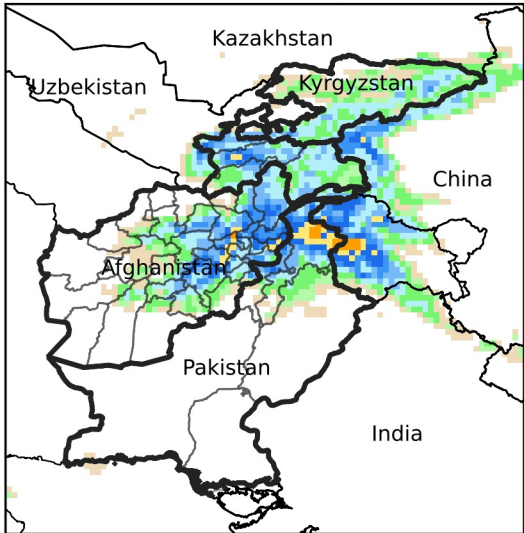
Daily Precip. Forecast for May 1, 2024
