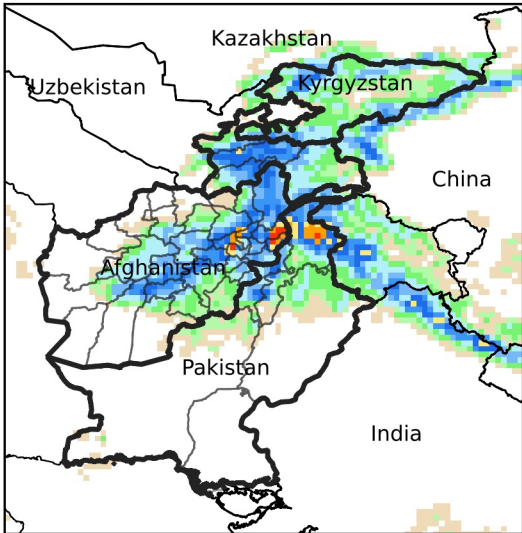
Daily Precip. Forecast for Apr 30, 2024
