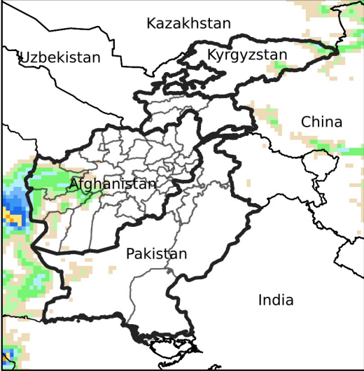
Daily Precip. Forecast for May 2, 2024
