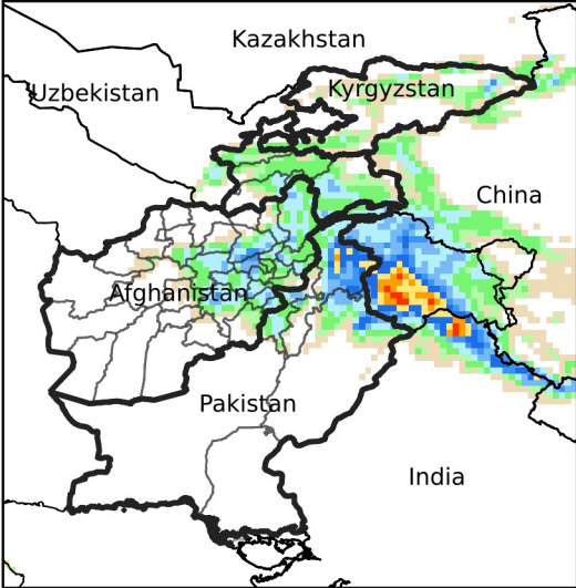
Daily Precip. Forecast for May 2, 2024
