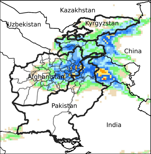
Daily Precip. Forecast for May 1, 2024
