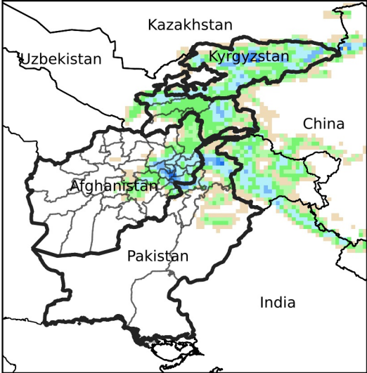
Daily Precip. Forecast for May 3, 2024
