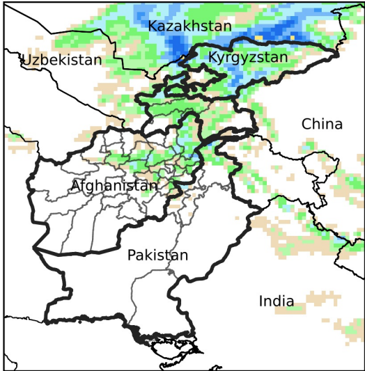
Daily Precip. Forecast for May 5, 2024
