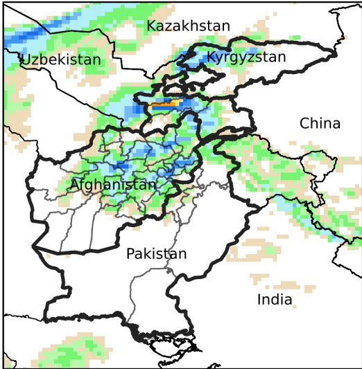
Daily Precip. Forecast for May 4, 2024
