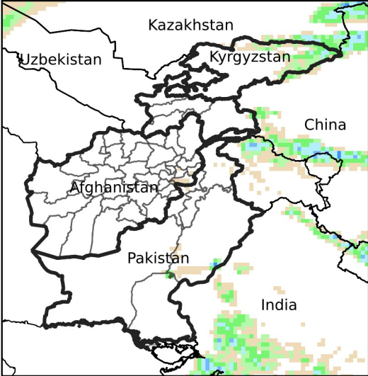
Daily Precip. Forecast for May 16, 2024
