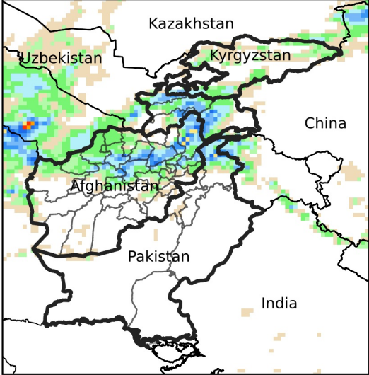
Daily Precip. Forecast for May 17, 2024
