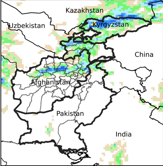
Daily Precip. Forecast for May 16, 2024
