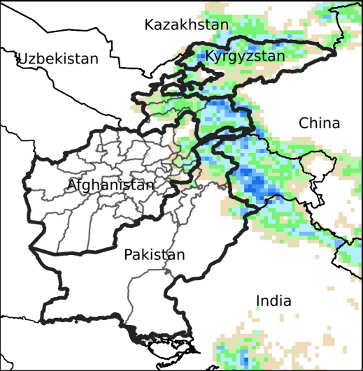
Daily Precip. Forecast for May 15, 2024
