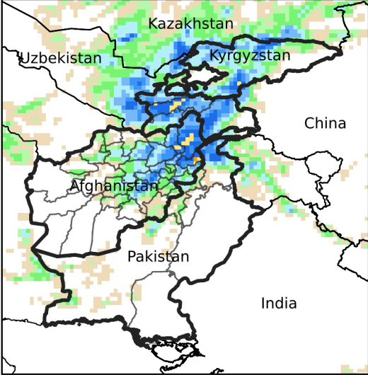
Daily Precip. Forecast for May 18, 2024
