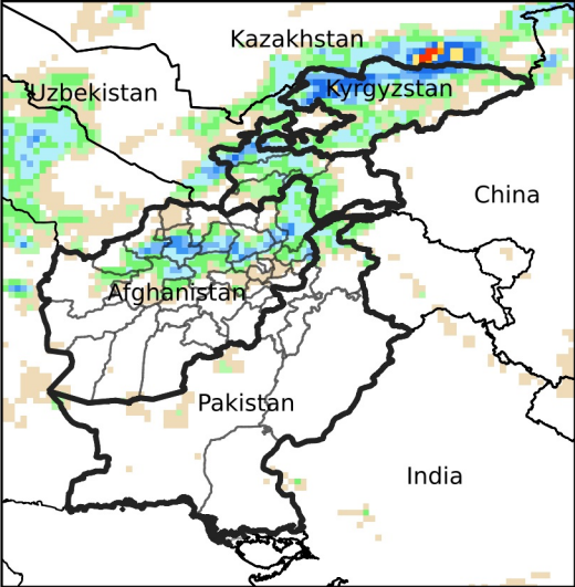
Daily Precip. Forecast for May 19, 2024
