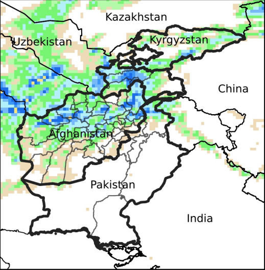
Daily Precip. Forecast for May 17, 2024
