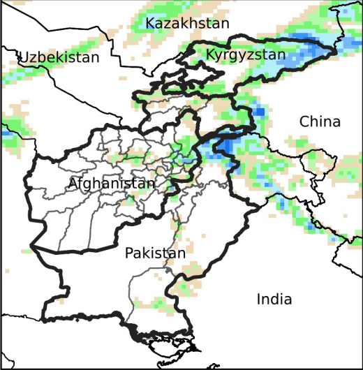
Daily Precip. Forecast for May 19, 2024
