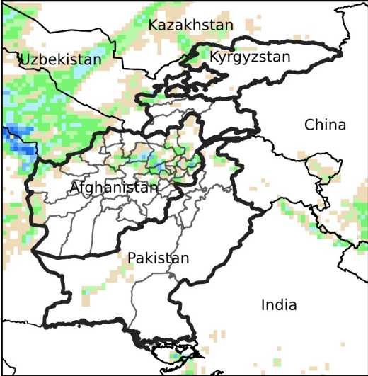
Daily Precip. Forecast for May 18, 2024
