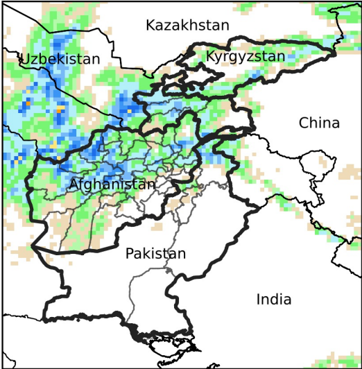
Daily Precip. Forecast for May 20, 2024
