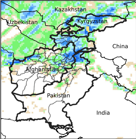
Daily Precip. Forecast for May 21, 2024
