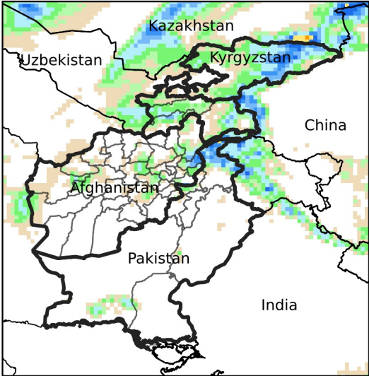
Daily Precip. Forecast for May 22, 2024
