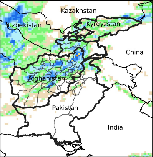
Daily Precip. Forecast for May 20, 2024
