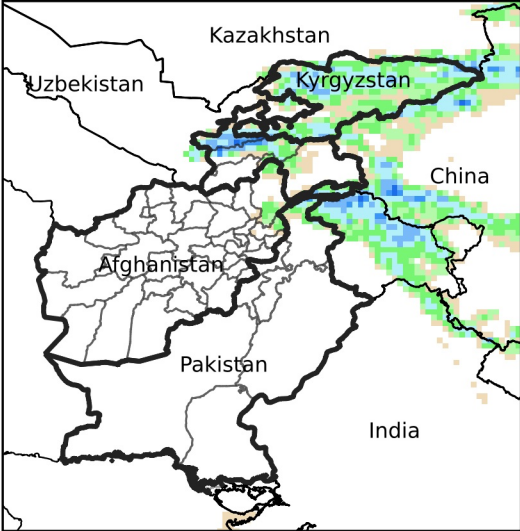
Daily Precip. Forecast for Jun 2, 2024
