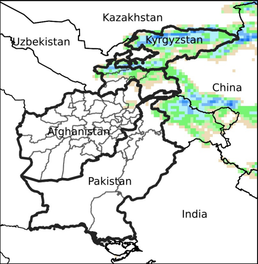
Daily Precip. Forecast for Jun 1, 2024
