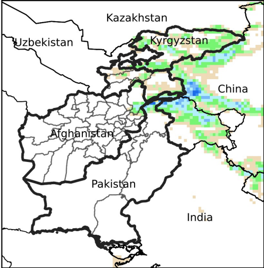
Daily Precip. Forecast for Jun 3, 2024
