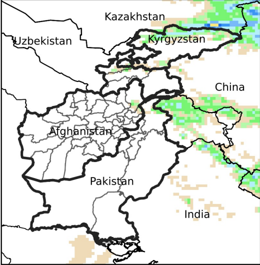
Daily Precip. Forecast for Jun 2, 2024
