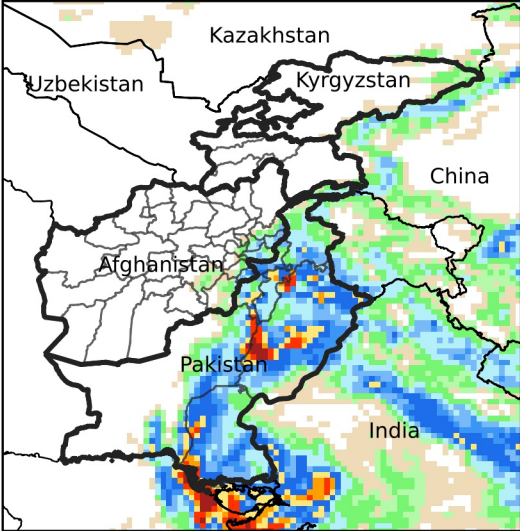
Daily Precip. Forecast for Aug 30, 2024
