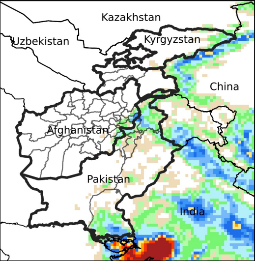
Daily Precip. Forecast for Aug 29, 2024
