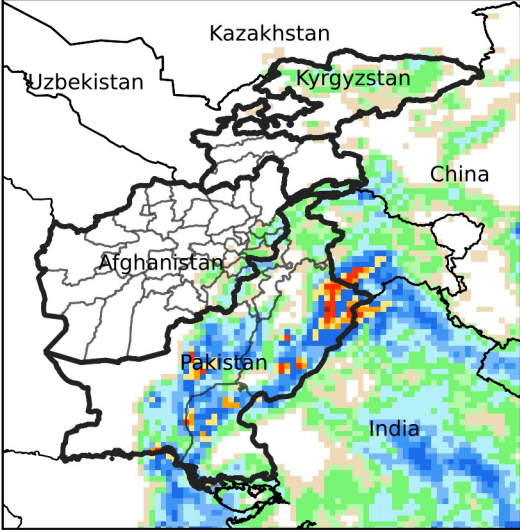
Daily Precip. Forecast for Aug 30, 2024
