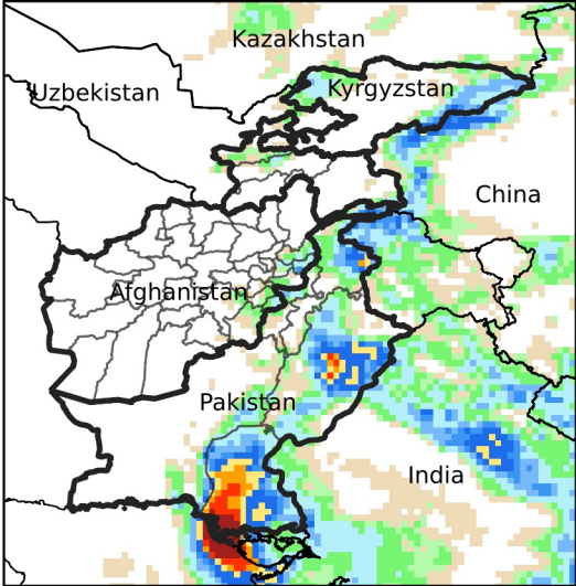
Daily Precip. Forecast for Aug 31, 2024
