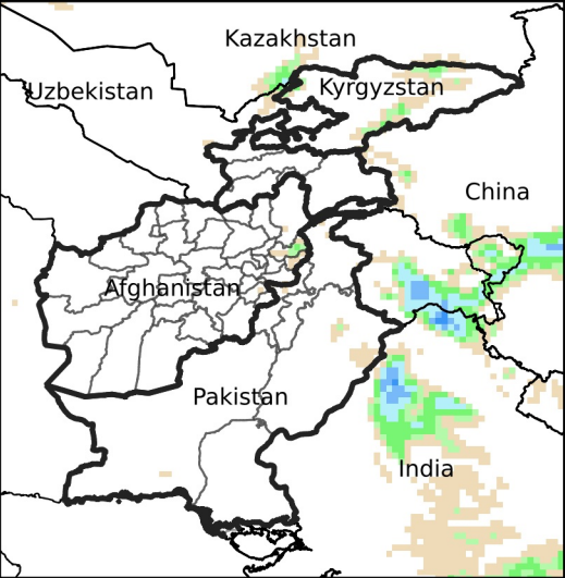
Daily Precip. Forecast for Sep 22, 2024
