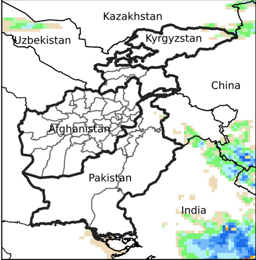
Daily Precip. Forecast for Sep 24, 2024
