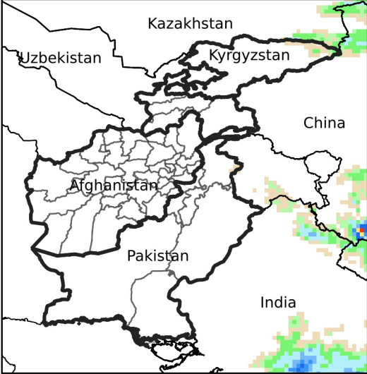
Daily Precip. Forecast for Sep 23, 2024
