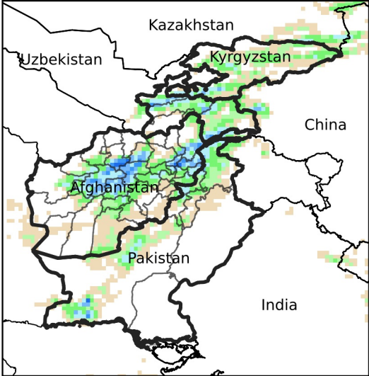
Daily Precip. Forecast for Oct 10, 2024
