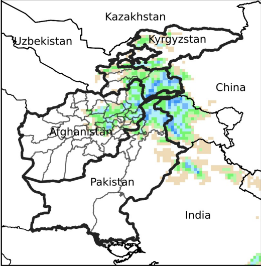
Daily Precip. Forecast for Oct 9, 2024
