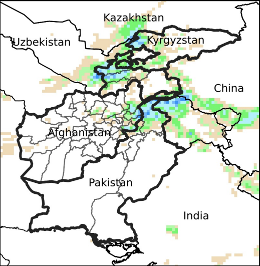
Daily Precip. Forecast for Oct 8, 2024
