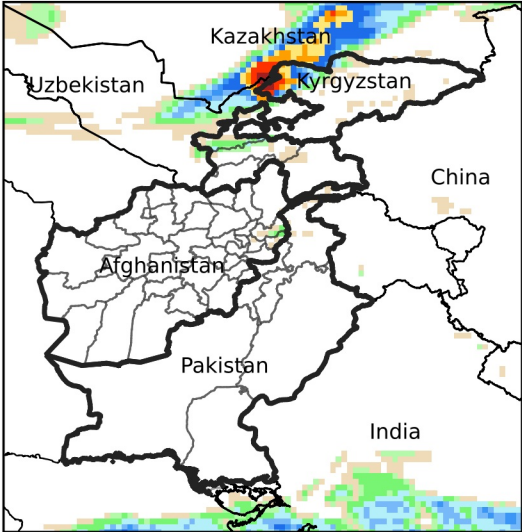
Daily Precip. Forecast for Oct 17, 2024
