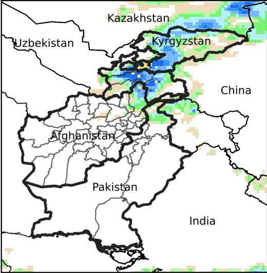
Daily Precip. Forecast for Oct 16, 2024
