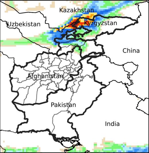
Daily Precip. Forecast for Oct 15, 2024
