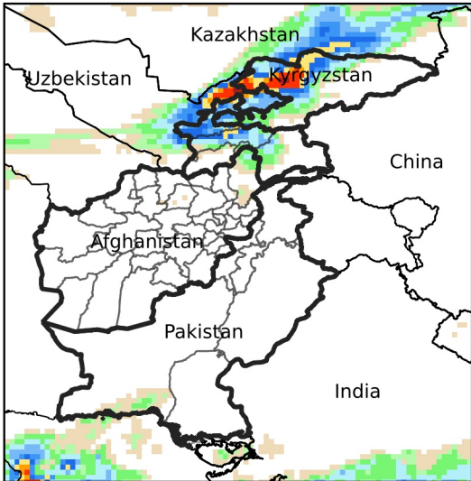
Daily Precip. Forecast for Oct 18, 2024
