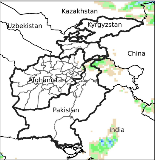
Daily Precip. Forecast for Oct 17, 2024
