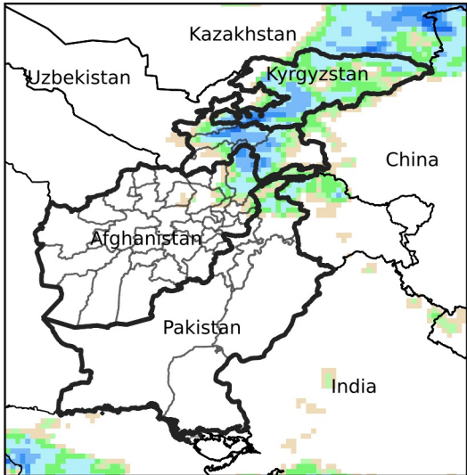
Daily Precip. Forecast for Oct 19, 2024
