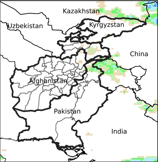
Daily Precip. Forecast for Oct 20, 2024
