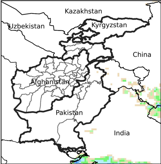
Daily Precip. Forecast for Oct 22, 2024
