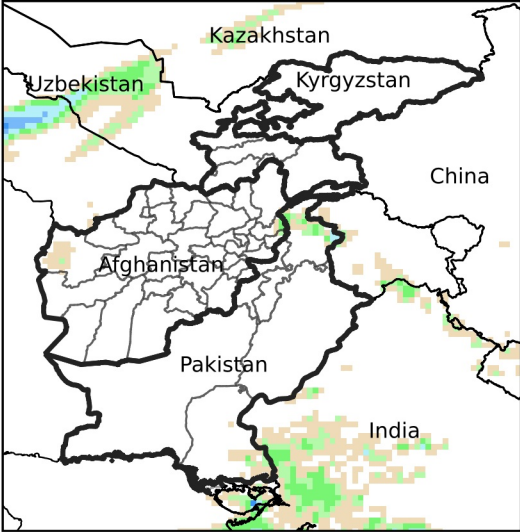
Daily Precip. Forecast for Oct 21, 2024
