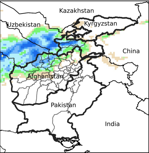
Daily Precip. Forecast for Oct 25, 2024
