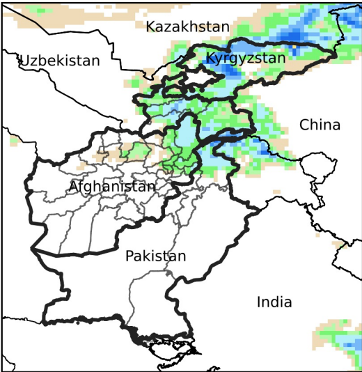
Daily Precip. Forecast for Oct 31, 2024
