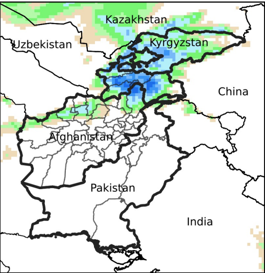
Daily Precip. Forecast for Oct 30, 2024
