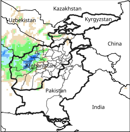
Daily Precip. Forecast for Nov 28, 2024
