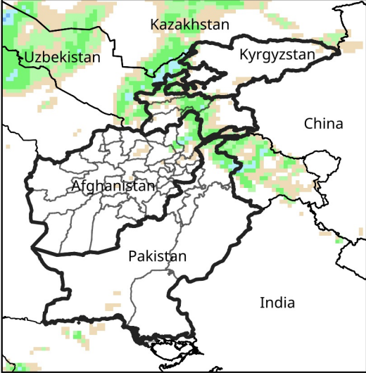
Daily Precip. Forecast for Nov 30, 2024
