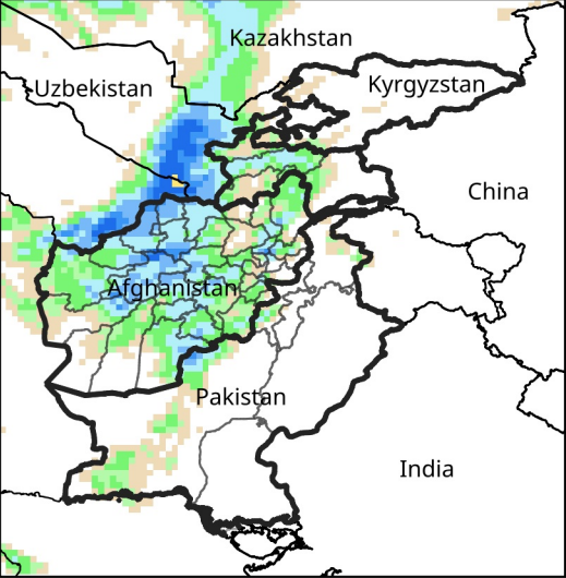
Daily Precip. Forecast for Nov 29, 2024
