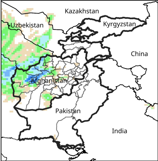
Daily Precip. Forecast for Dec 1, 2024
