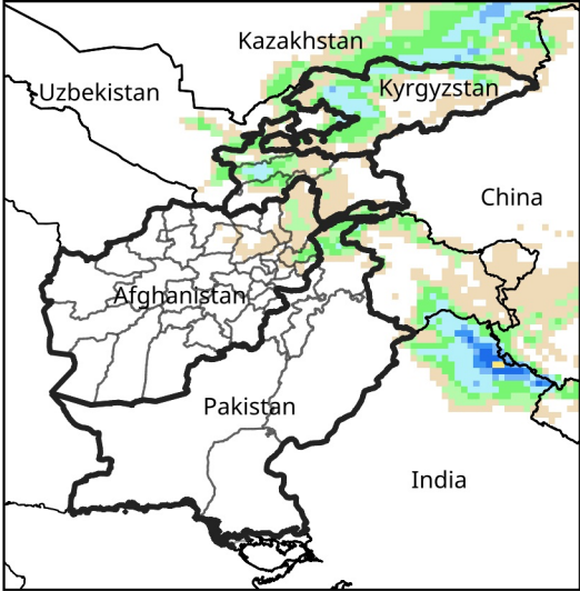
Daily Precip. Forecast for Dec 8, 2024
