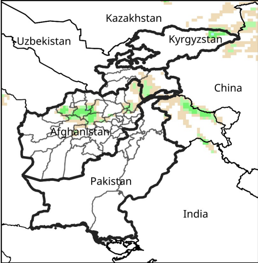
Daily Precip. Forecast for Dec 13, 2024
