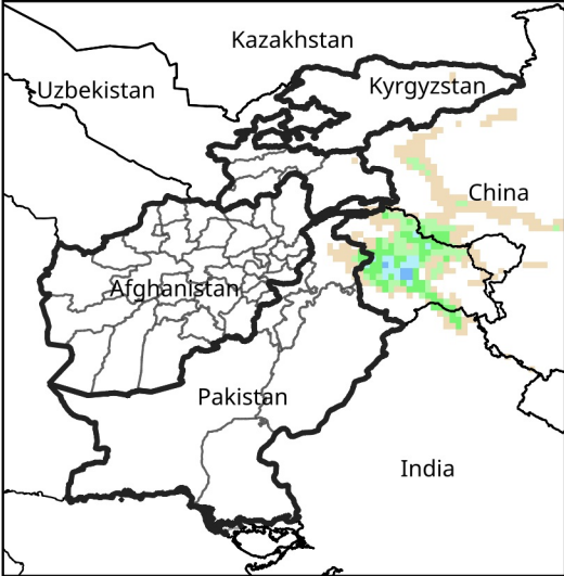
Daily Precip. Forecast for Dec 15, 2024
