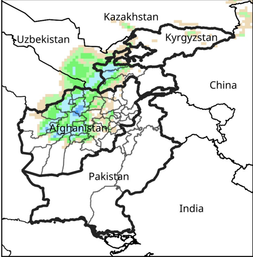
Daily Precip. Forecast for Dec 16, 2024
