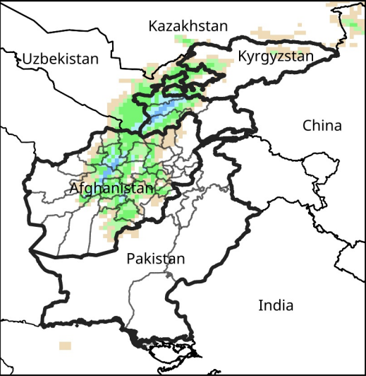
Daily Precip. Forecast for Dec 16, 2024
