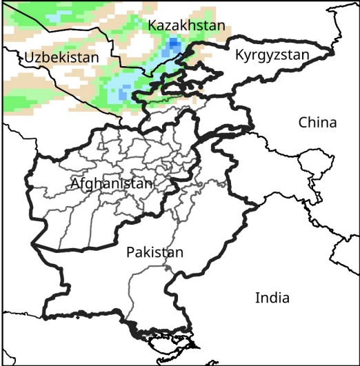
Daily Precip. Forecast for Dec 22, 2024
