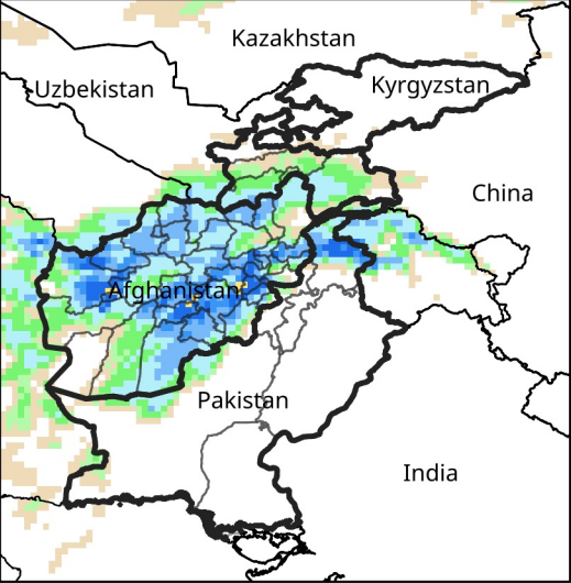
Daily Precip. Forecast for Jan 2, 2025
