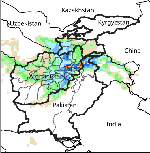
Daily Precip. Forecast for Jan 3, 2025
