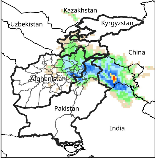
Daily Precip. Forecast for Jan 5, 2025
