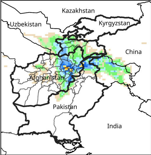
Daily Precip. Forecast for Jan 7, 2025
