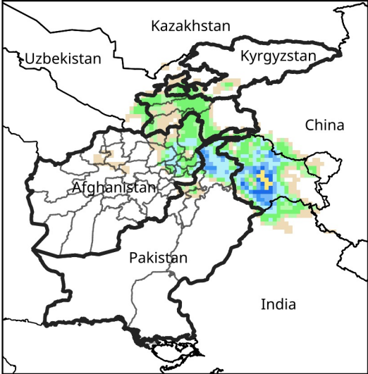
Daily Precip. Forecast for Jan 8, 2025
