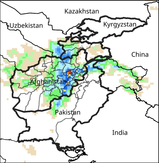
Daily Precip. Forecast for Jan 6, 2025
