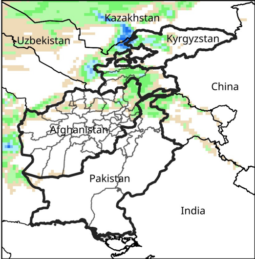
Daily Precip. Forecast for Jan 24, 2025
