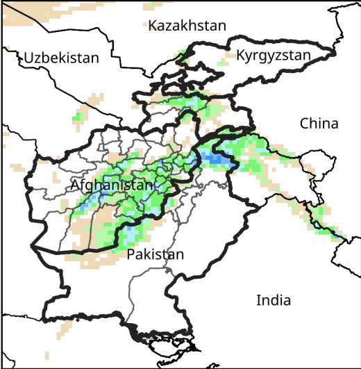
Daily Precip. Forecast for Jan 23, 2025
