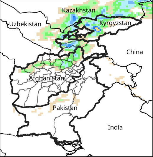
Daily Precip. Forecast for Jan 22, 2025
